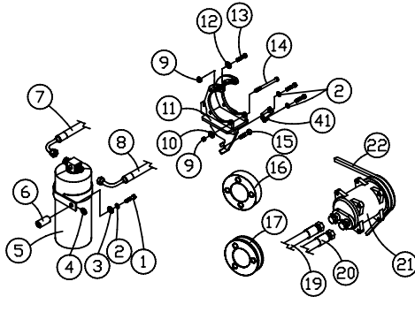
COMPRESSOR ASSEMBLY
