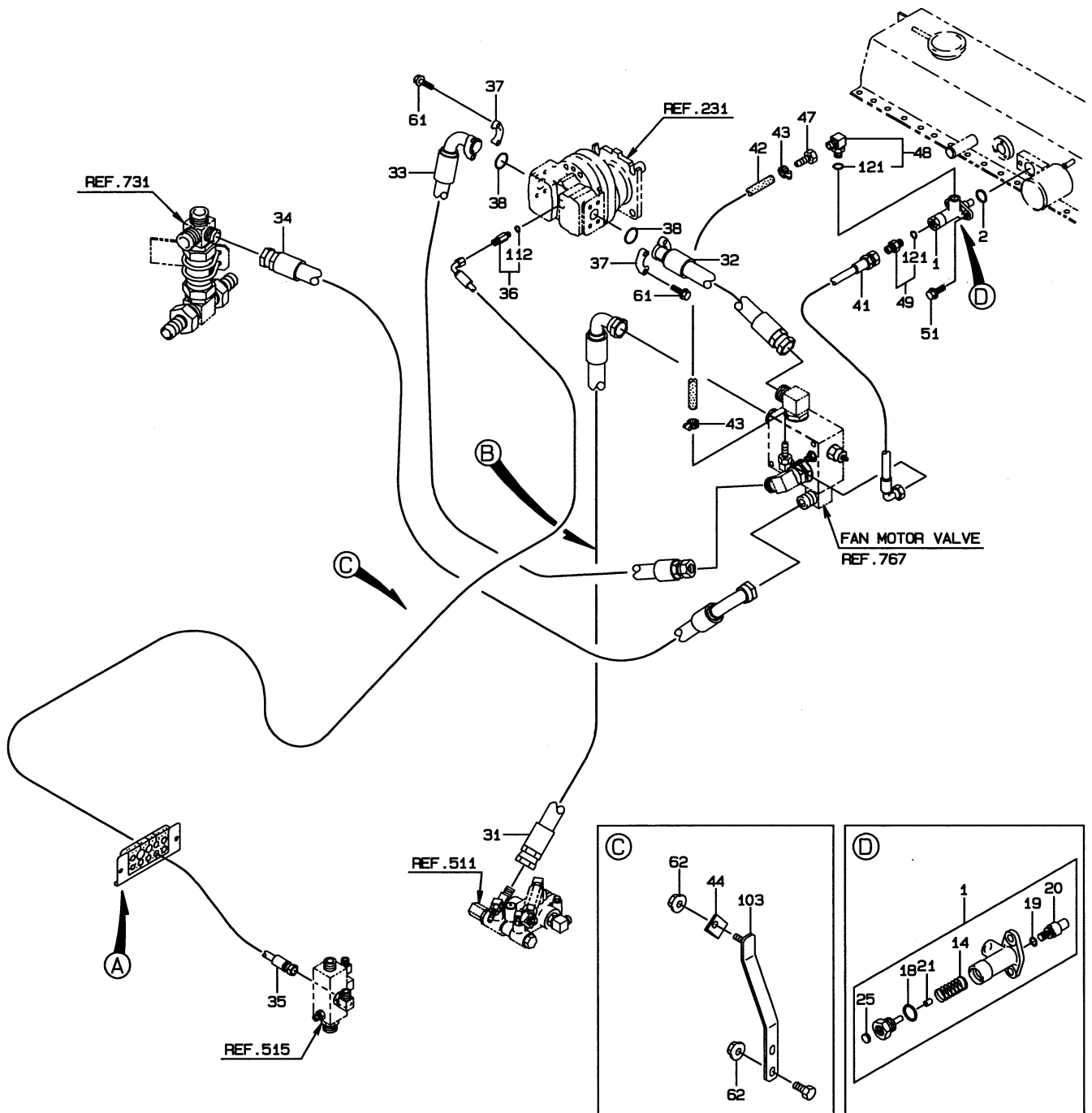
DETAIL OF PIPE HOLDER
