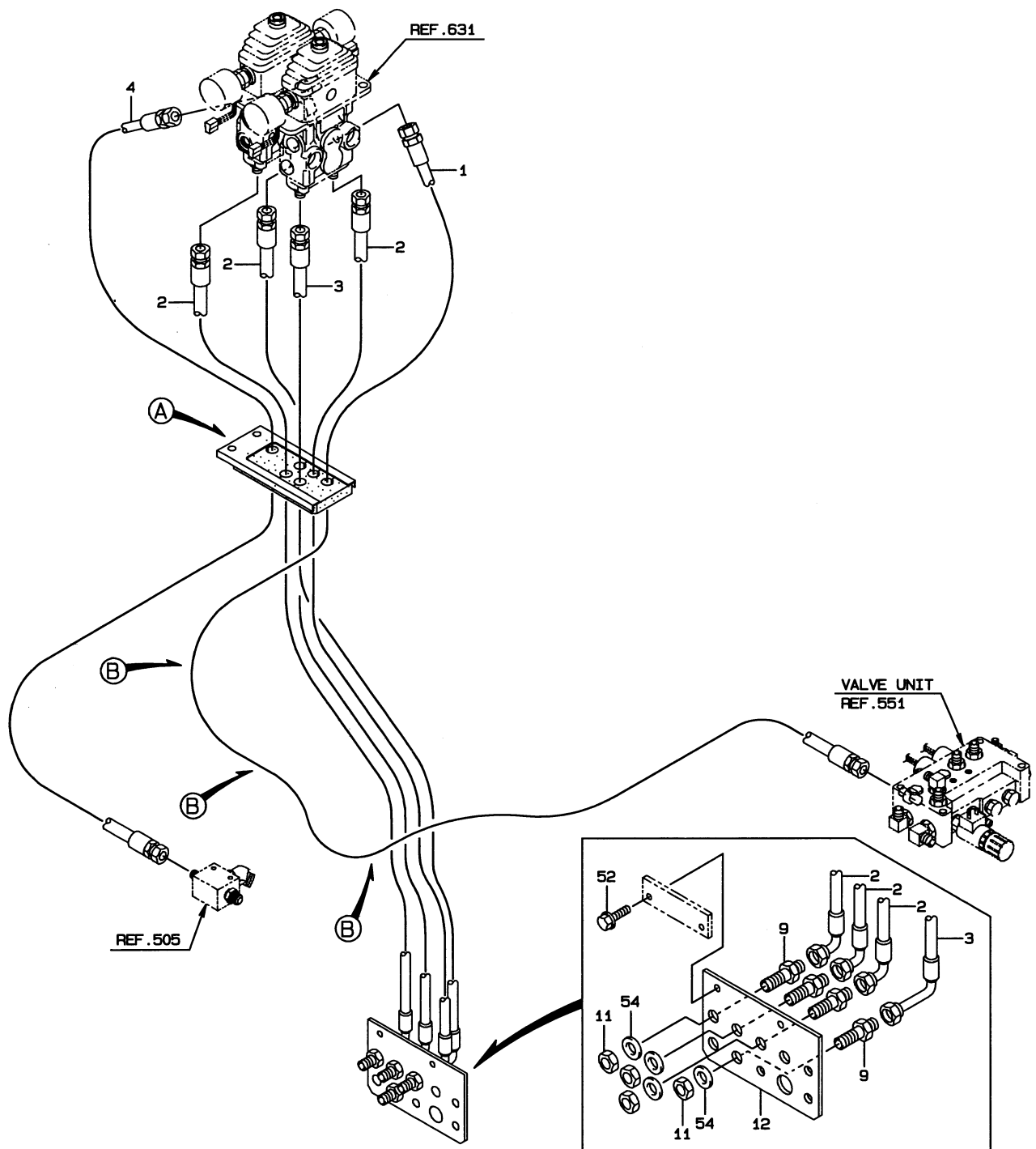
DETAIL OF PIPE HOLDER
