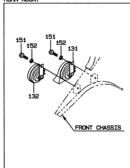
HORN MOUNT
