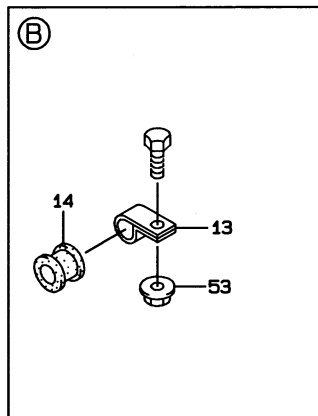
DETAIL OF PIPE HOLDER
