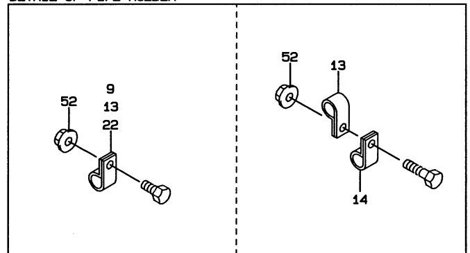
DETAIL OF PIPE HOLDER
