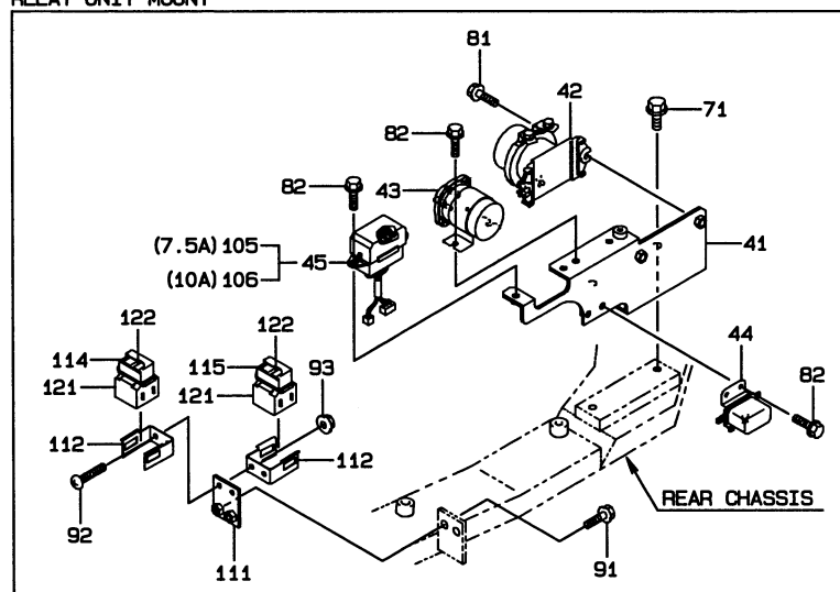
RELAY UNIT MOUNT
