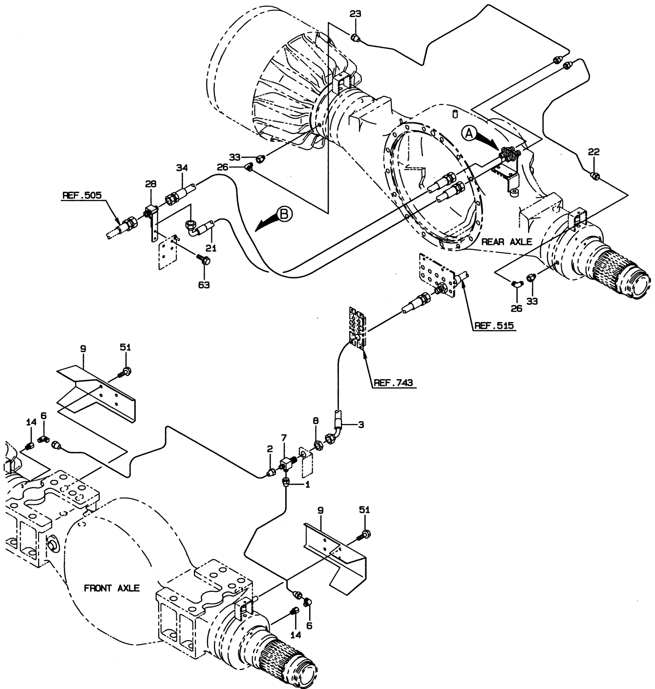
DETAIL OF PIPE HOLDER
