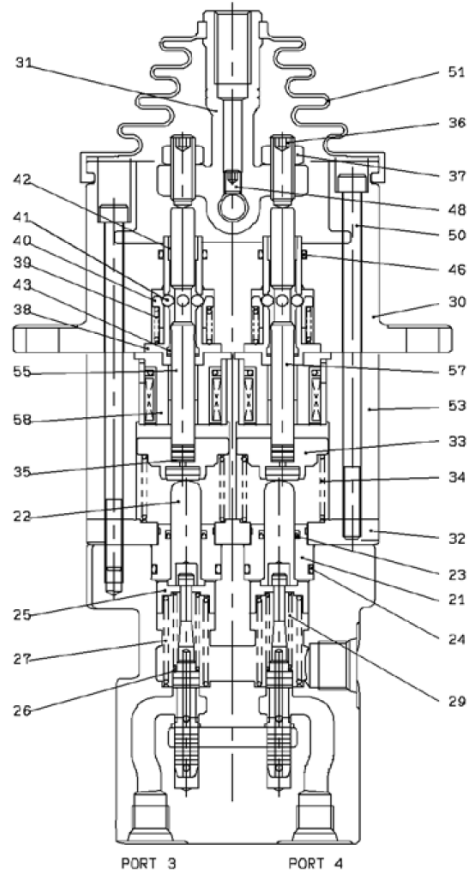
SECTION B-B
