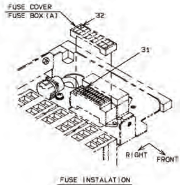
FUSE INSTALLATION
