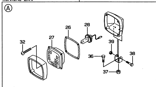
作業灯 WORKING LAMP
