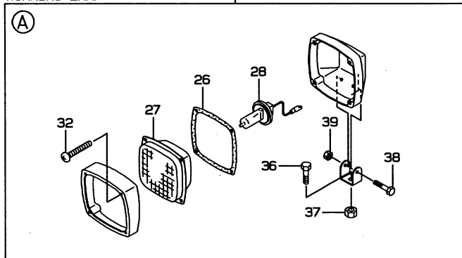
作業灯 WORKING LAMP
