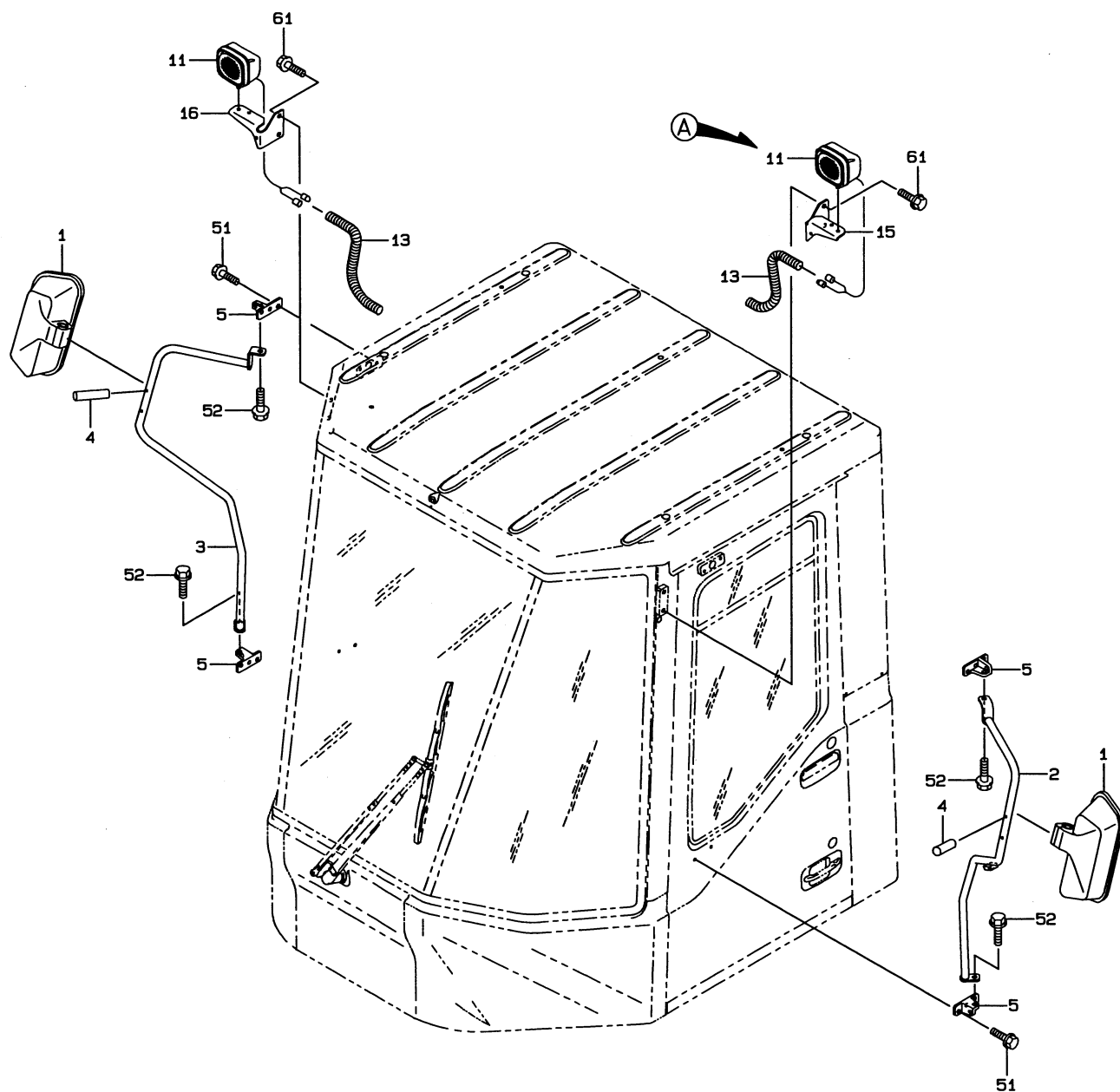
作業灯 WORKING LAMP
