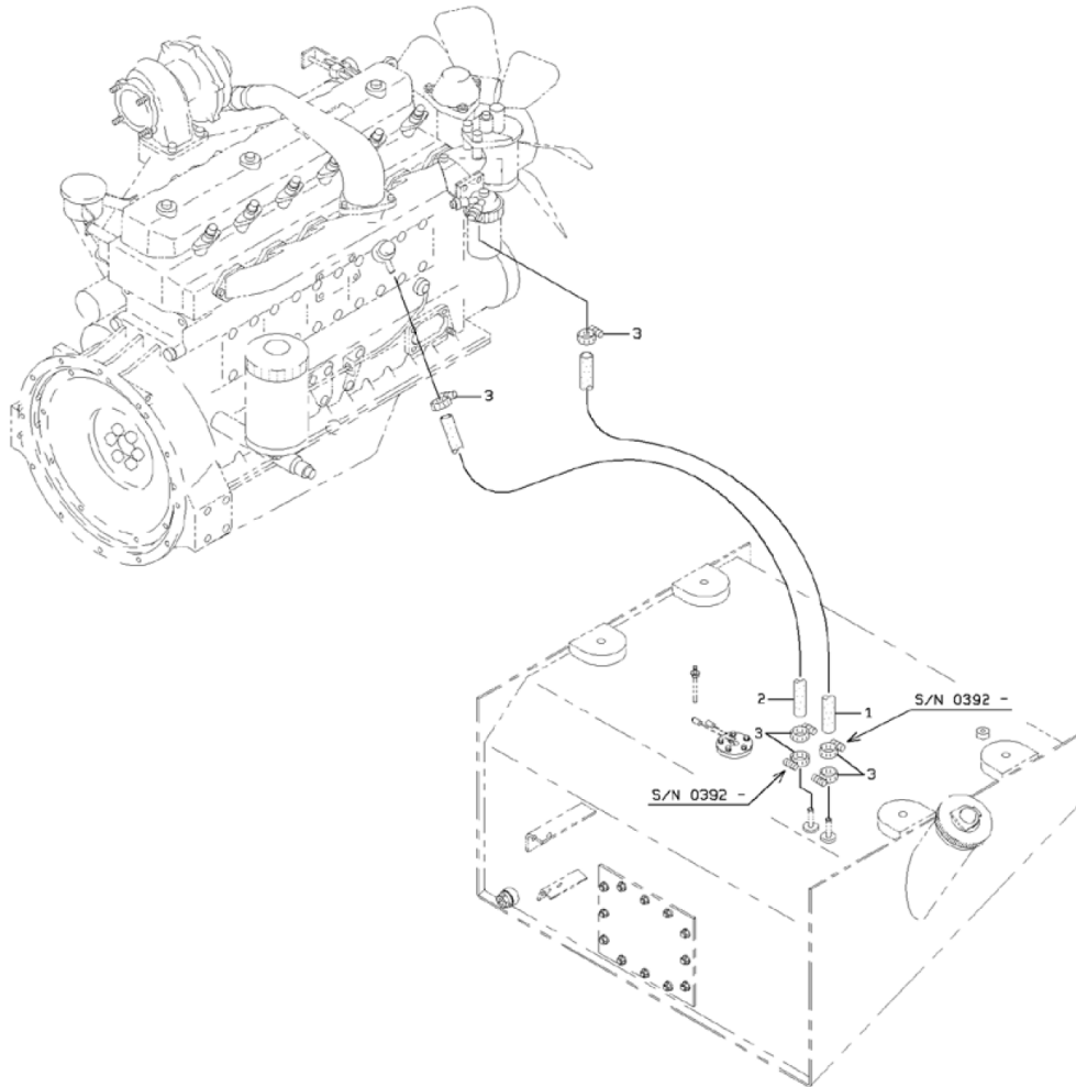
DETAIL OF PIPE HOLDER
