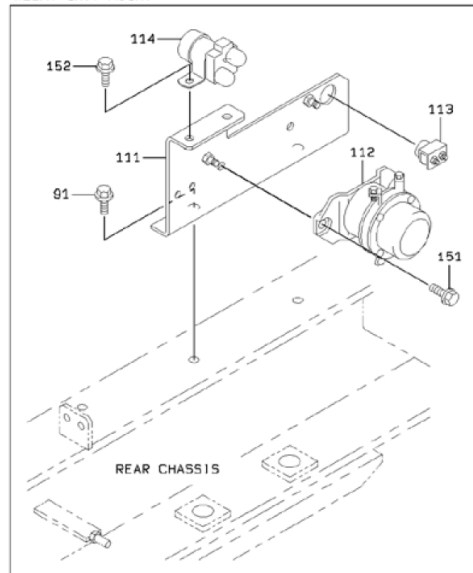
RELAY UNIT MOUNT
