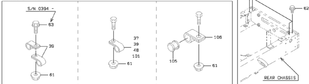
DETAIL OF PIPE HOLDER
