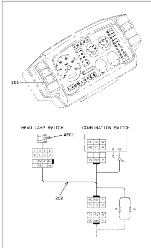
HEAD LAMP SWITCH MOUNT
