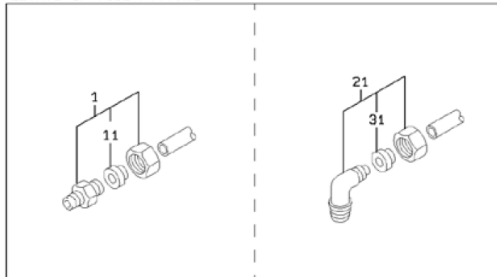
DETAIL OF TUBE FITTING
