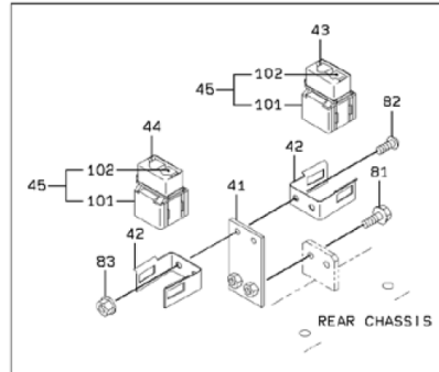
SLOW BLOW FUSE MOUNT
