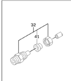
DETAIL OF TUBE FITTING
