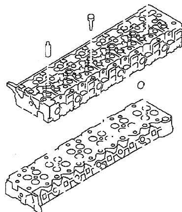
CYLINDER HEAD
