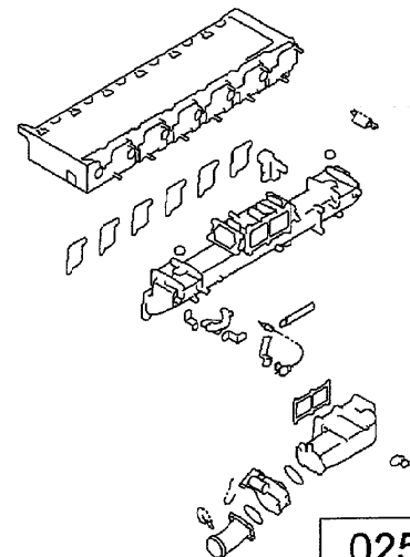
INLET MANIFOLD
