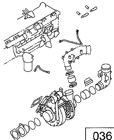
TURBOCHARGER SYSTEM
