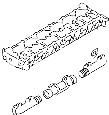
THERMOSTAT AND HOUSING
