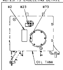
#2, 23, 73 LABELLING DETAIL
