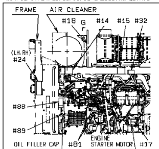
#14, 15, 17, 24, 32, 81, 88, 89 LABELLING DETAIL
