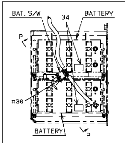
VIEW N-N
